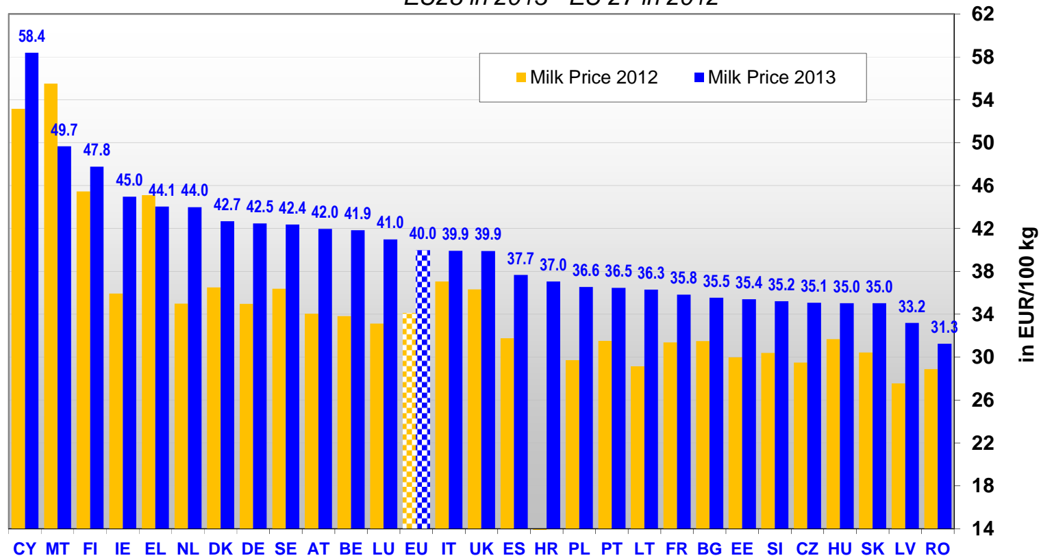
EU Milk Prices (November 2013 compared to November 2012) EU28 in 2013 - EU 27 in 2012
